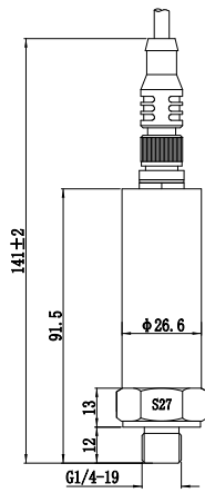
RS485型-M12航插出线
