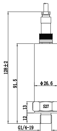
RS485型-Gx12航插出线
